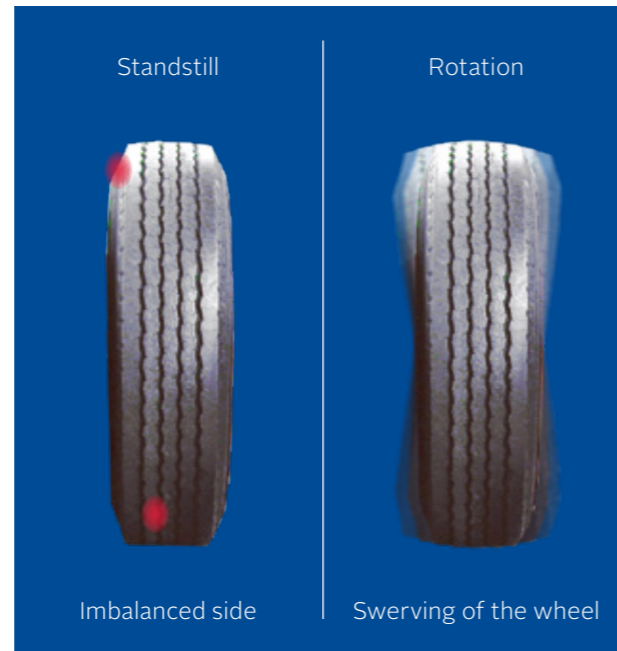
DYNAMIC IMBALANCE
